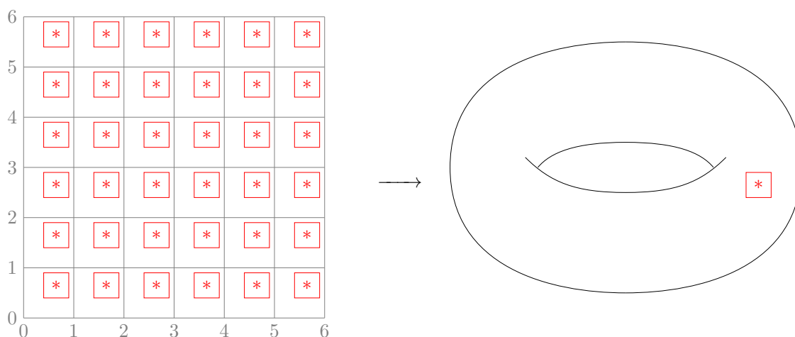
Abbildung 3.11: \mathbb{R}^2 \rightarrow T^2 = \mathbb{R}^2 / \mathbb{Z}^2
